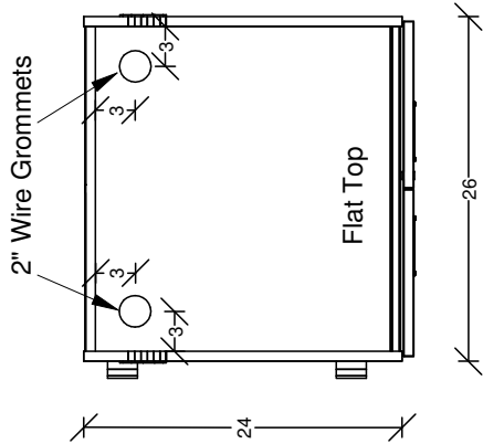
TYPICAL PLAN VIEW
