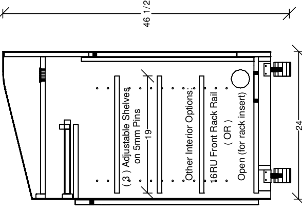
TYPICAL CUT SECTION
