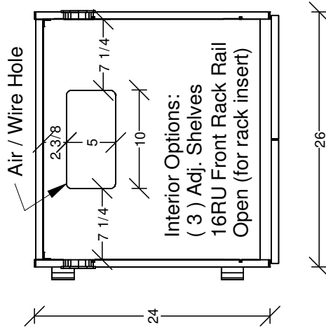
TYPICAL PLAN @ BOTTOM
